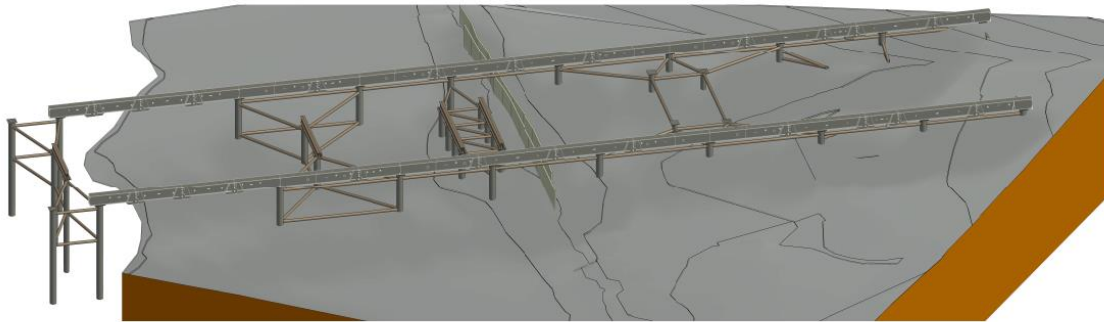
2 ISOMETRIC VIEW 2
